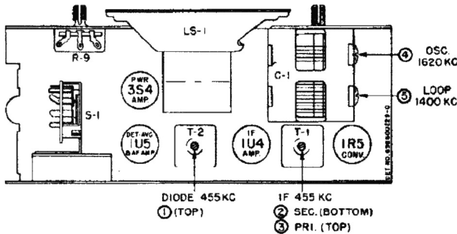
FIGURE 2. TUBE & TRIMMER LOCATIONS REPLACEMENT PARTS LIST
