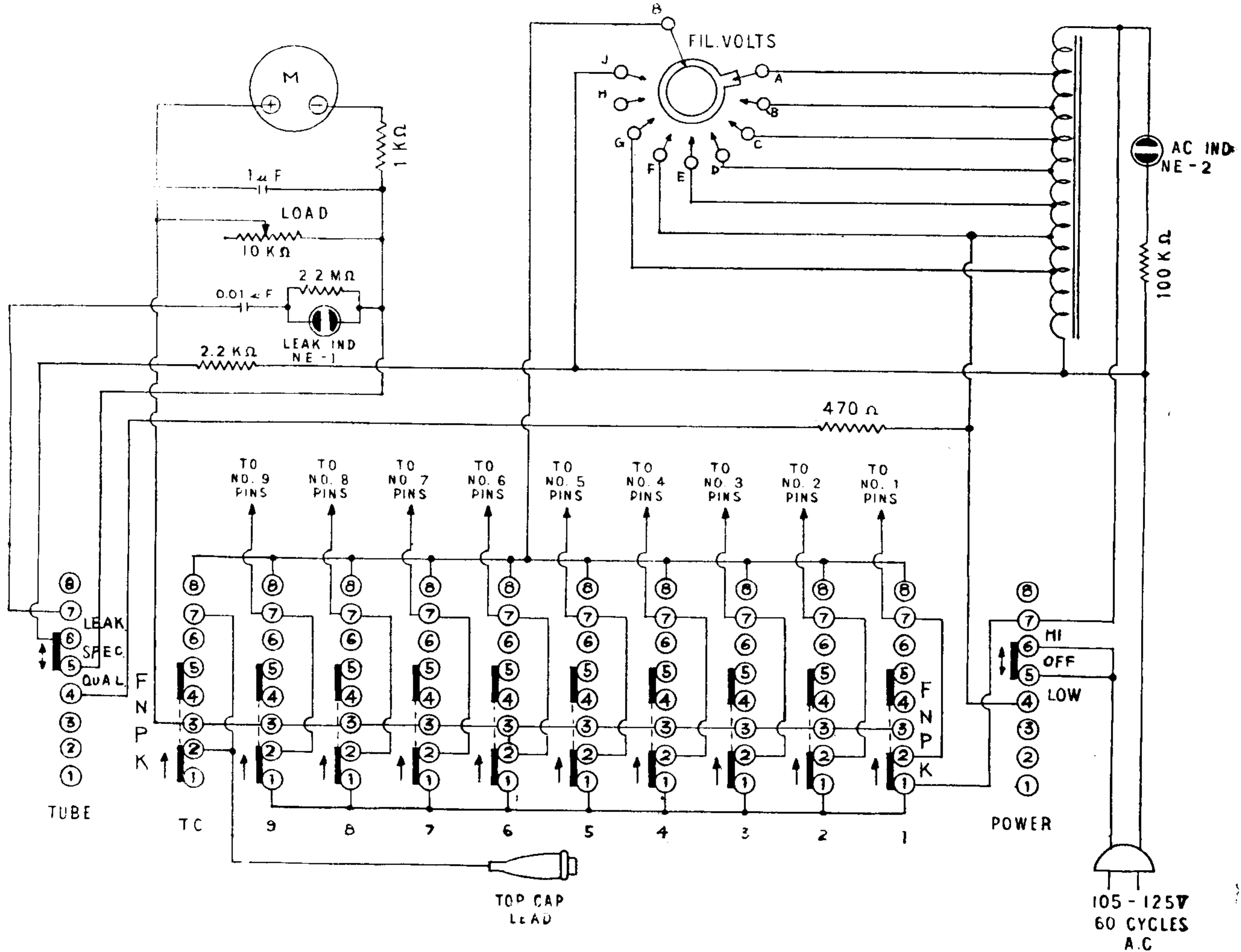
SCHMATIC DIAGRAM
